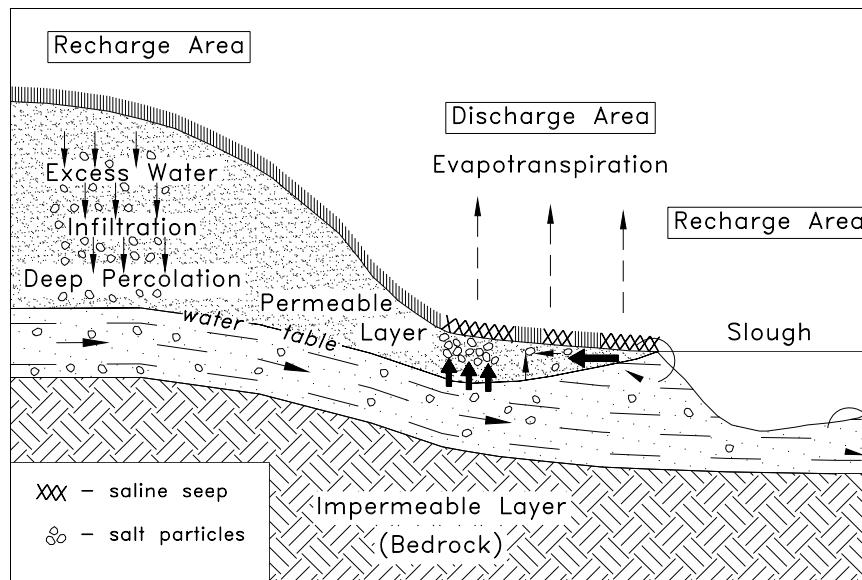
Figure 1. Generalized saline seep mechanisms
