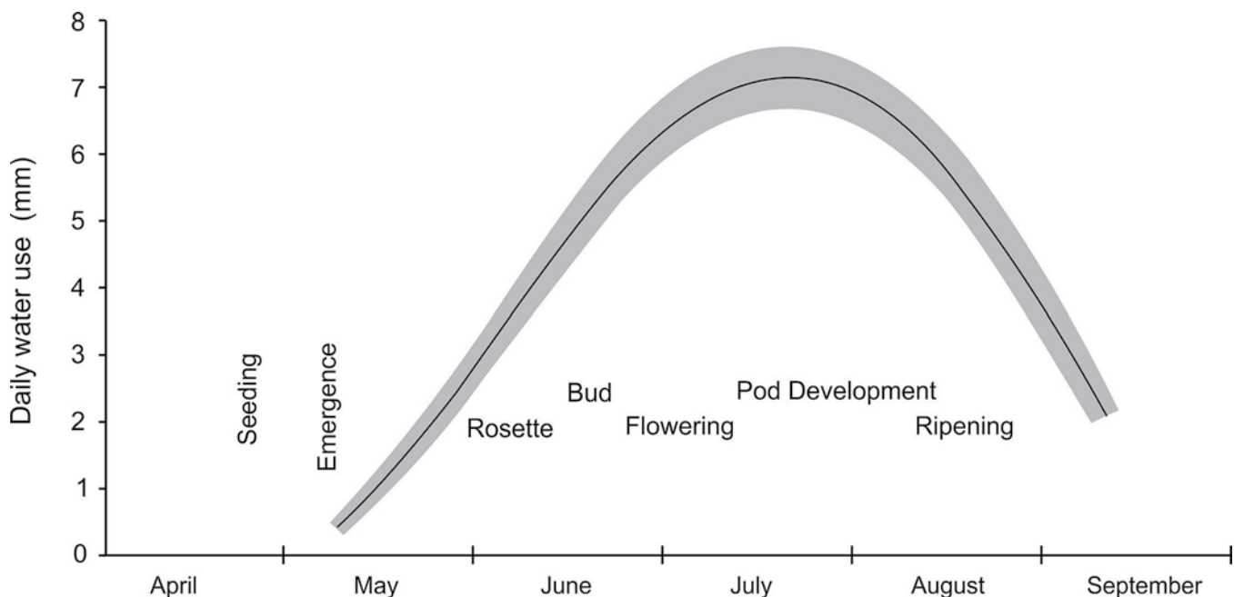
Figure 1. Daily water use during different growth stages of irrigated canola in southern Alberta. Shaded area indicates variation in canola water use depending on plant type, cultivar, and climatic conditions.
