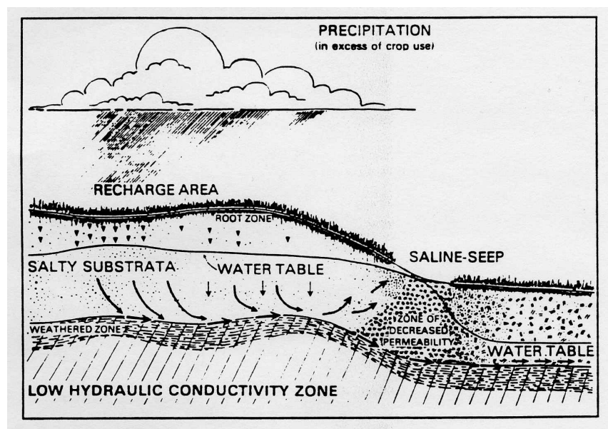
Figure 1. Generalised diagram of saline seep, recharge area, and the substrata formation that contributes to a saline seep (Brown et al. 1982)
