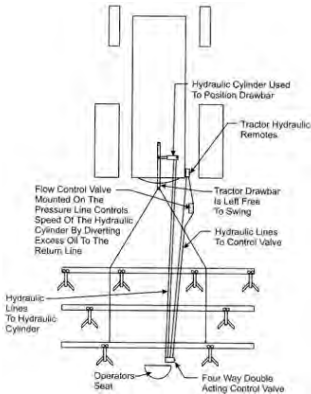
Figure 8. Concept for operator assist, hydraulically controlled guidance system.
