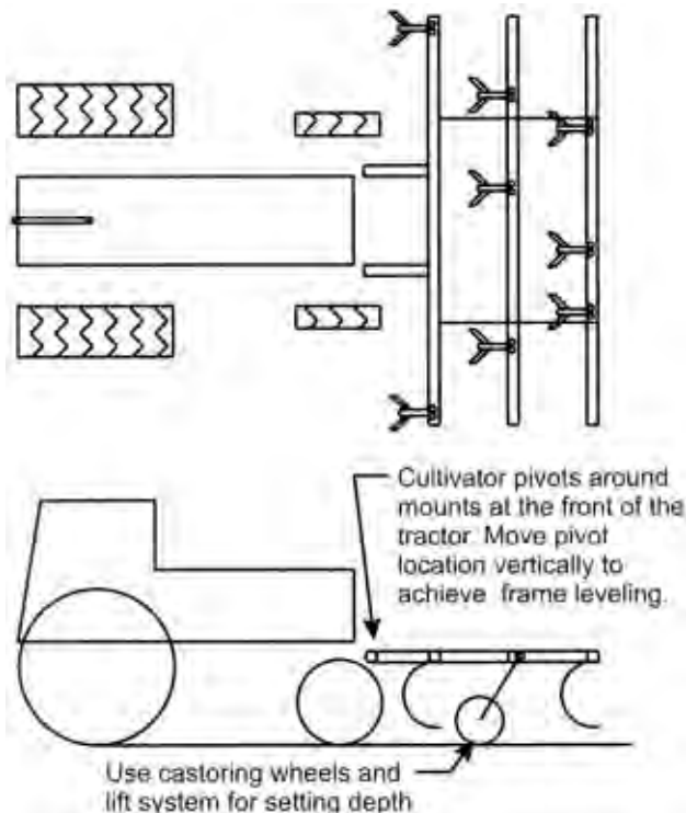
Figure 2. Push cultivator mounted in front of tractor.
