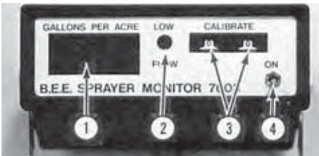
FIGURE 3. BEE Meter: (1) Application Rate Display Screen, (2) Low Flow Indicator Light, (3) Calibration Thumbwheel Switches, (4) On-Off Power Switch.
