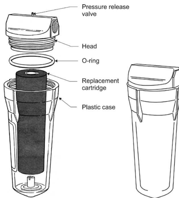
Figure 1. Activated carbon (taste and odour)
