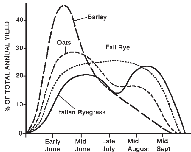
Figure 5. Typical seasonal distribution of pasture yield*.
