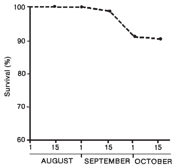
Figure 2. Influence of seeding date on per cent winter survival of rye grown in north-central Saskatchewan.
