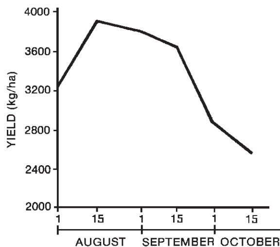
Figure 1. Influence of seeding date on yield of rye produced on summer fallow (mean of five trials).
