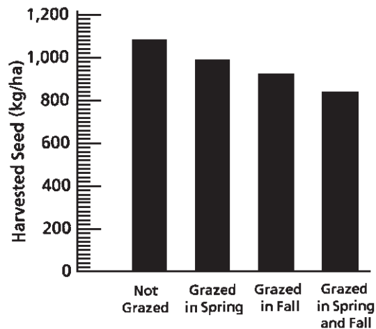
Figure 4. An average effect of grazing on subsequent grain yields.
