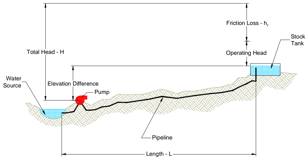
Pumped Pipeline - Example
